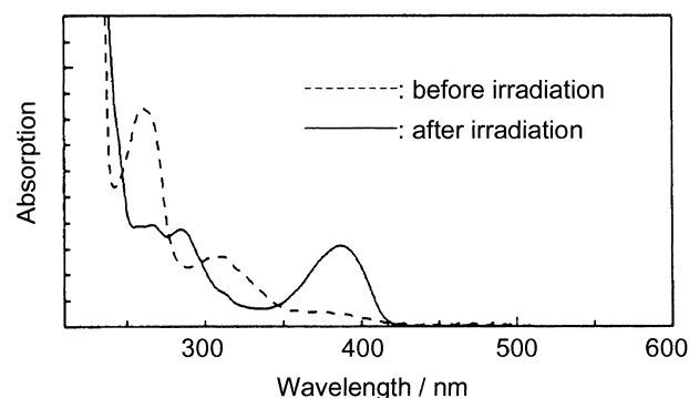
Fig. 3. Absorption spectral changes before and after photolysis of 1a in a 2-MeTHF matrix in 77 K.
