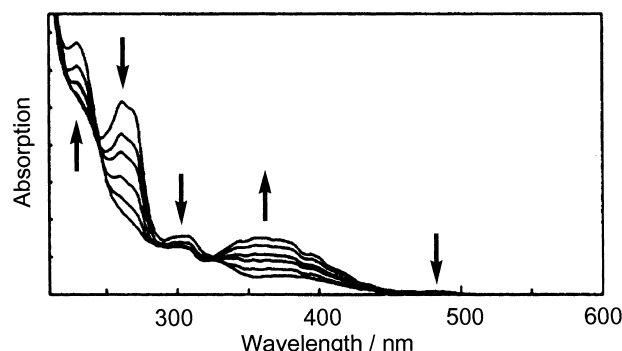
Fig. 2. Changes of absorption spectra of 1a in a 3-MP matrix at 77 K during photolysis.
