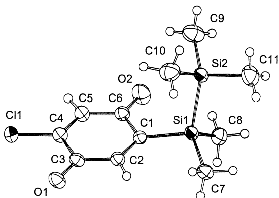
Fig. 1. ORTEP drawing of 1a . Selected bond lengths ( \text{\AA} ): C11–C4 = 1.740(4), Si1–Si2 = 2.349(2), Si1–C1 = 1.92(4), O1–C3 = 1.223(6), O2–C6 = 1.219(7), C1–C2 = 1.348(7), C1–C6 = 1.497(7), C2–C3 = 1.475(7), C3–C4 = 1.487(7), C5–C6 = 1.480(7).
